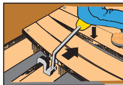
Hook tool on joist. Push handle down. Boards squeeze tight.
